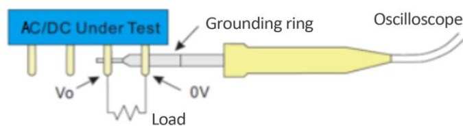
Diagram 4-3: Contact Measuring Method
