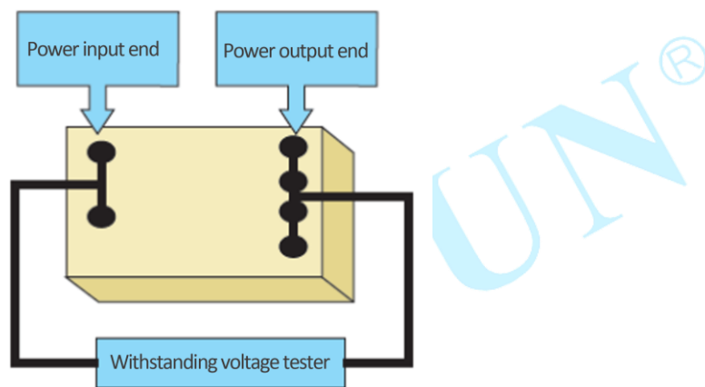
Diagram 4-7: Withstand Voltage Test
