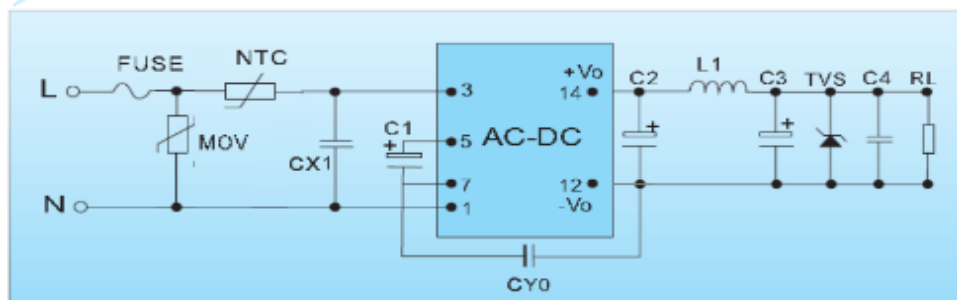
Diagram 4-5: LS Series Typical Circuit Diagram
