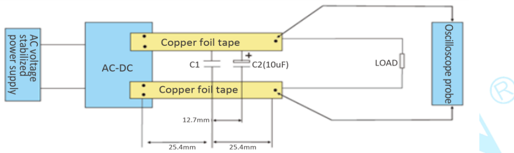
Diagram 4-1: Parallel Cable Measuring Method
