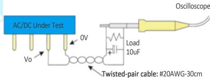
Diagram 4-2: Twisted-pair Cable Measuring Method
