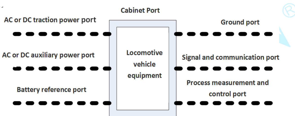
Fig.1. Locomotive Electrical Equipment Interfaces (ports)
