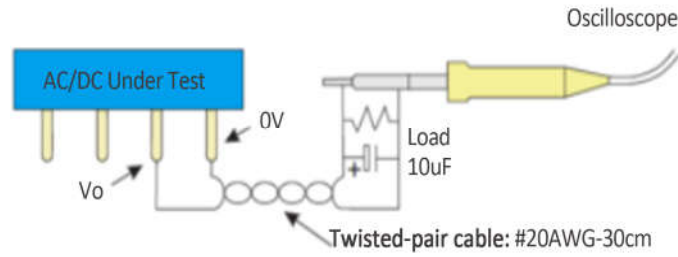
Diagram 4-2: Twisted-pair Cable Measuring Method
