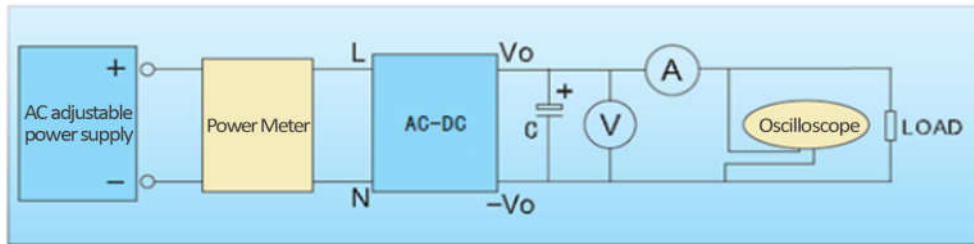
Diagram 3-1: Basic Test Circuit Connection
