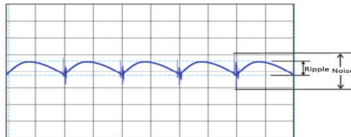
Diagram 4-4: Ripple & Noise Test Waveform
