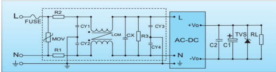
Diagram 3-3: Typical Input EMC Filter Circuit
