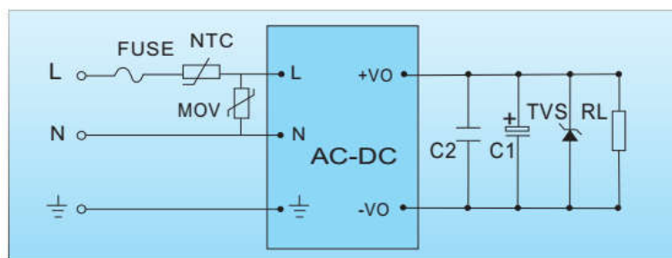
Diagram 3-2: General AC/DC Typical Application Circuit
